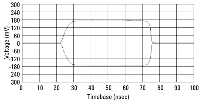
Measured pulse modulation envelope
